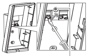
Wiring knockout
